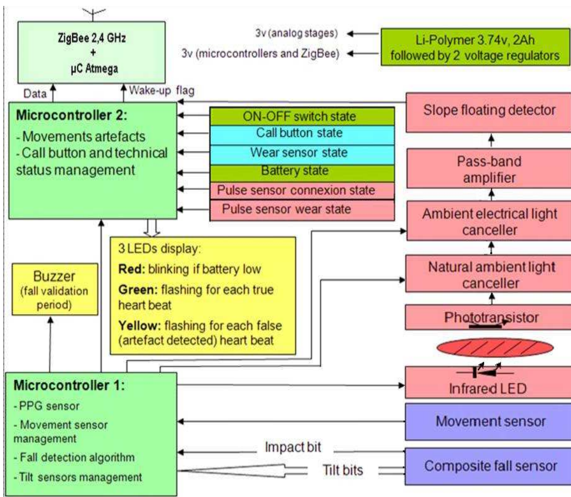
Fig. 3. Internal structure of the wearable device (RFpat)
