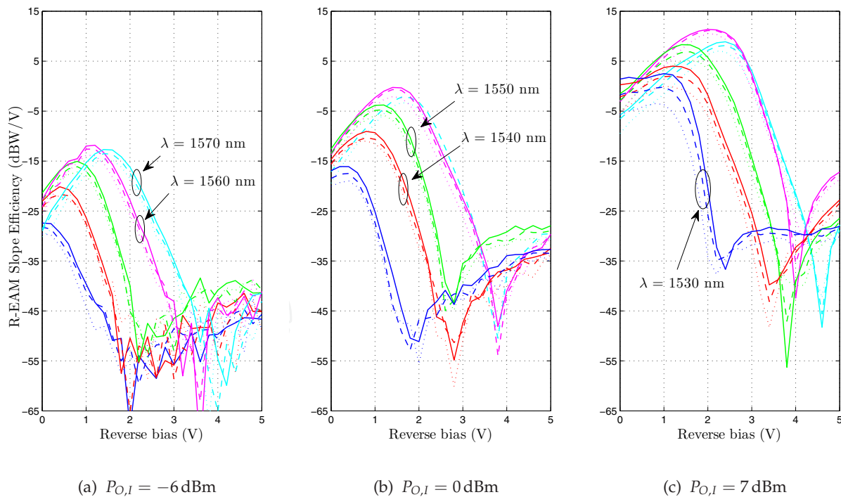
Figure 12. E/O response vs. reverse bias voltage for different wavelengths and frequencies and optical input powers. Solid, dashed and dotted lines correspond to frequencies of 2.4, 5, 15 GHz, respectively.
