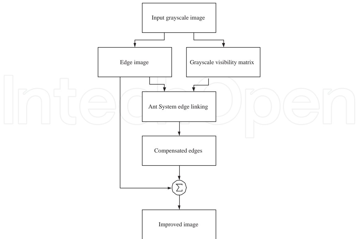
Figure 9. Block diagram of the proposed edge linking method
