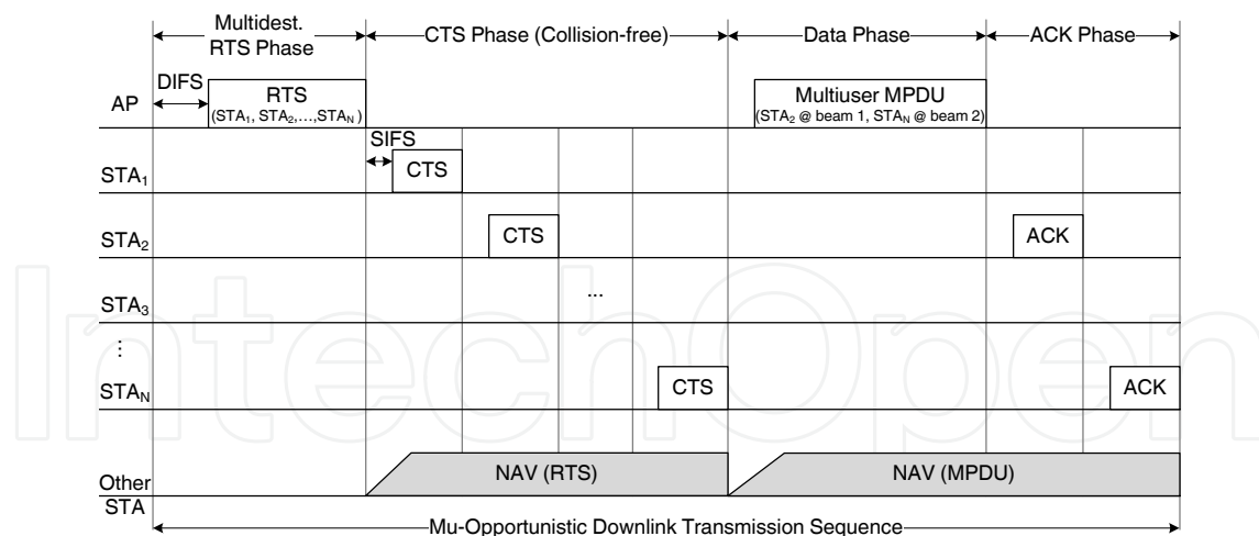
Figure 10. Transmission sequence example for the Mu-Opportunistic scheme
