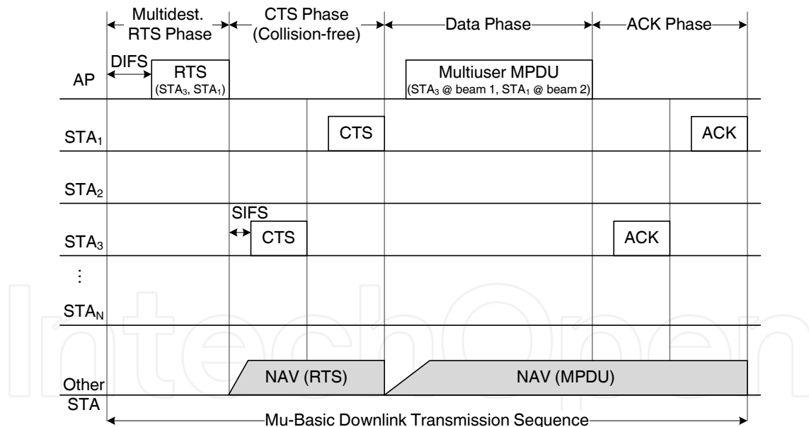
Figure 8. Transmission sequence example for the Mu-Basic scheme
