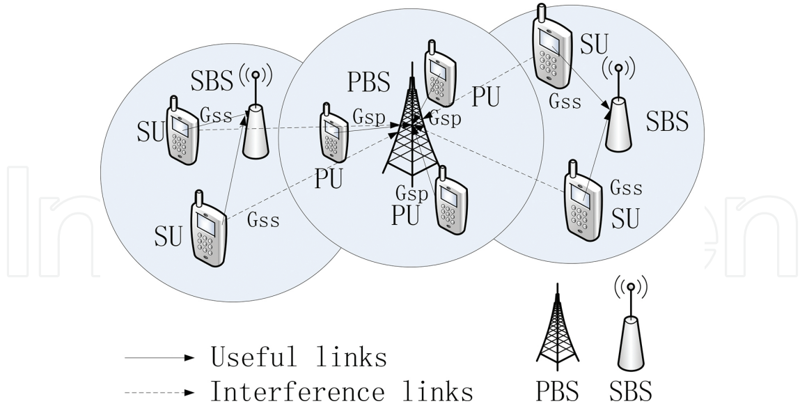
Figure 11. System model of two CR cells with multiple CR users per cell.
