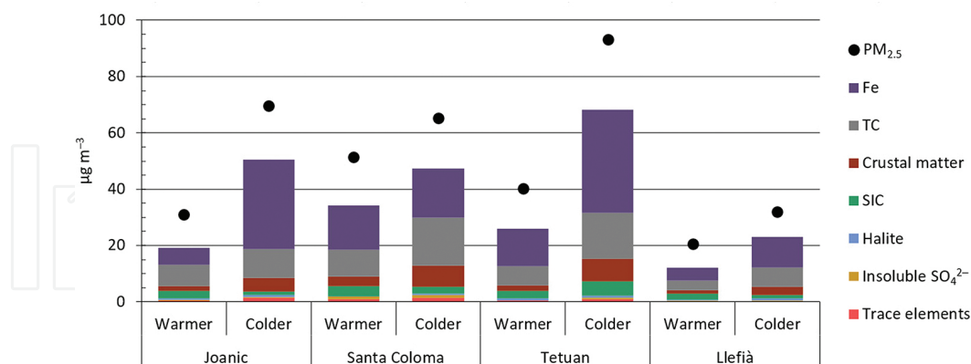
Figure 2. Mean concentrations of PM_{2.5} and the associated elemental components on the Joanic, Santa Coloma, Tetuan and Llefià platforms during the warmer and colder periods (TC, total carbon; SIC, secondary inorganic compounds).
