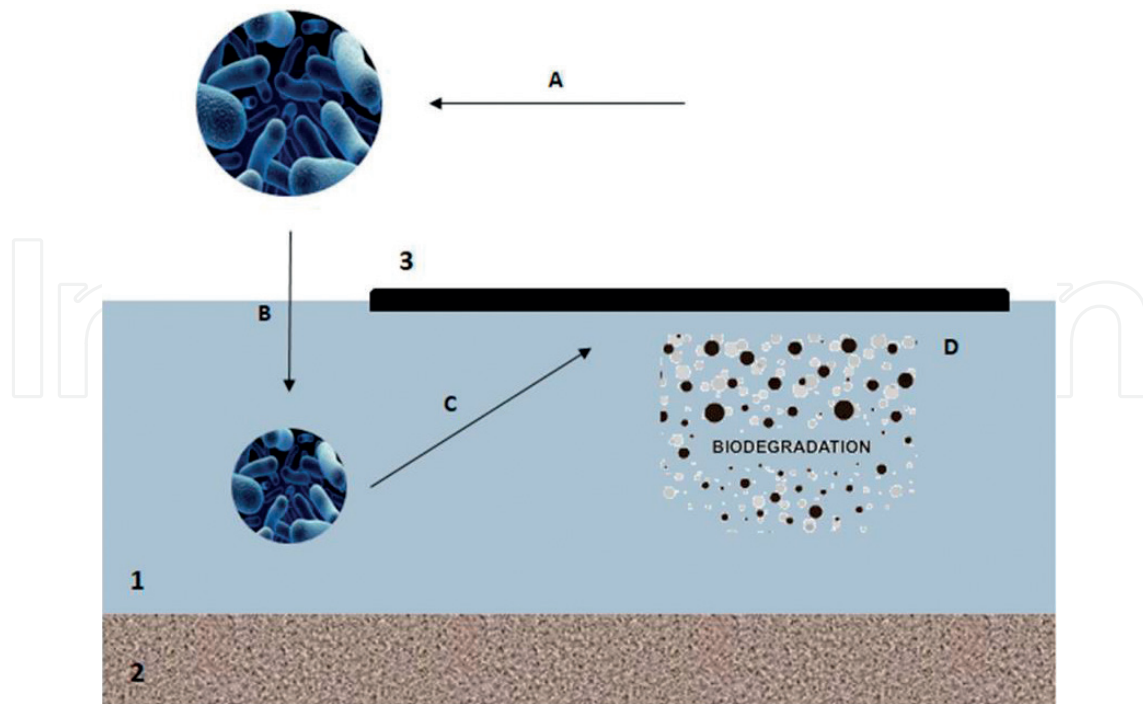
Figure 3. Schematic description of bioremediation (bioaugmentation) process. 1: Seawater; 2: marine sediment; 3: crude oil.
