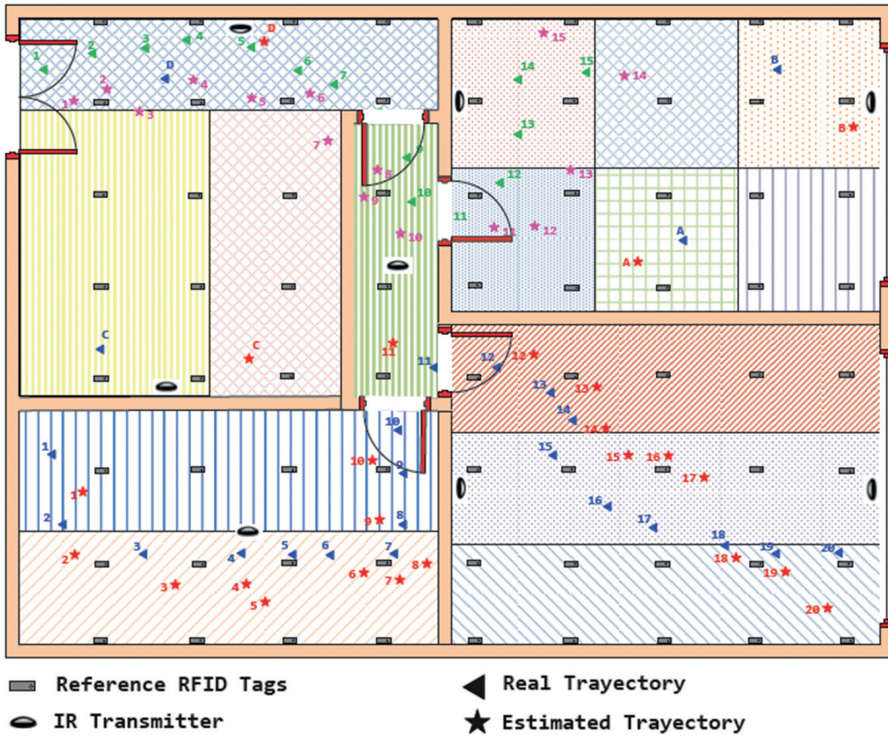
Figure 7.8 Tracking processes with a reference tag distribution of 1 m × 1 m.
