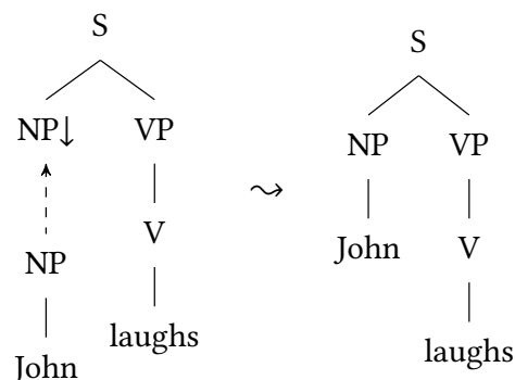
Figure 12.2: Substitution
