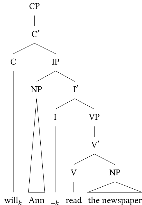
Figure 3.6: Polar question
