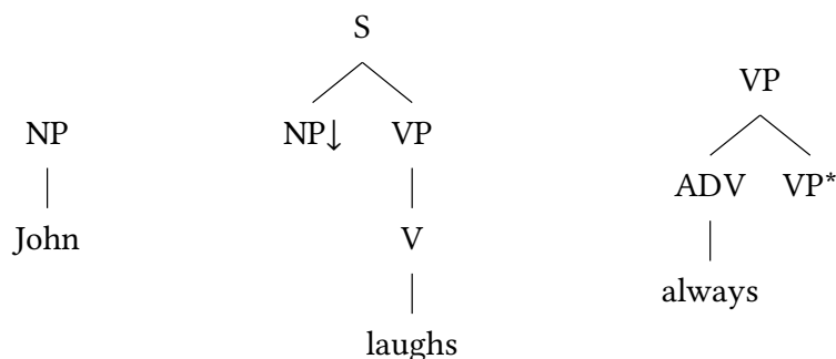
Figure 12.1: Elementary trees
