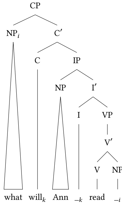
Figure 3.7: wh -question
