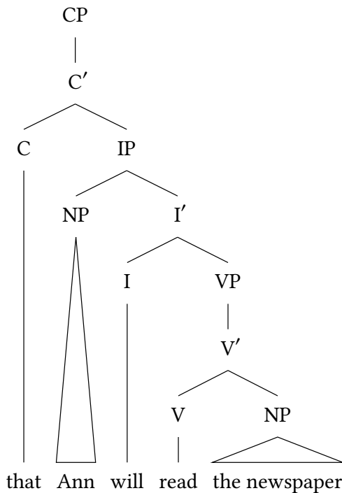
Figure 3.5: Complementizer phrase
