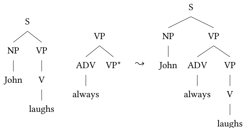
Figure 12.3: Adjunction
