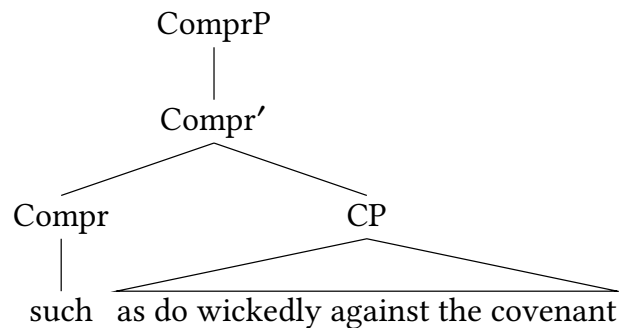
Figure 4.21: Equative relatives
