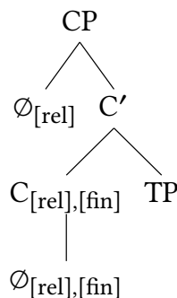
Figure 4.5: Zero relatives
