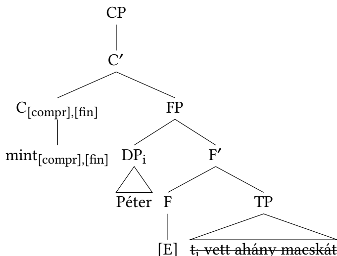
Figure 6.7: Elliptical comparatives
