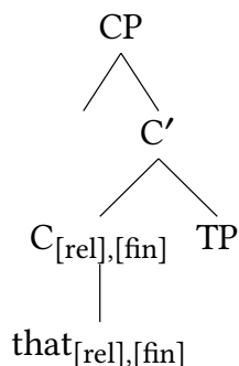
Figure 2.12: Relative complementisers
