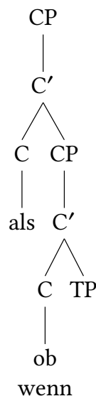
Figure 5.12: Hypothetical comparatives
