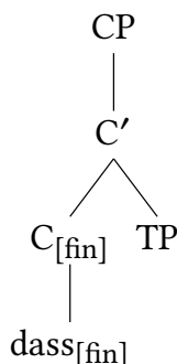
Figure 3.8: Embedded declaratives
