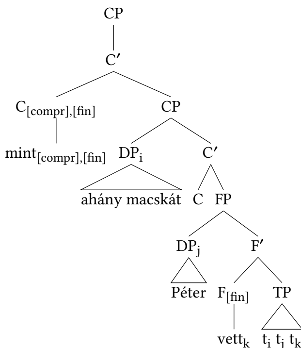
Figure 6.6: Comparative subclauses
