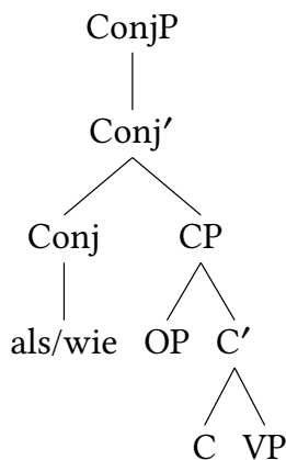
Figure 5.8: The ConjP-analysis
