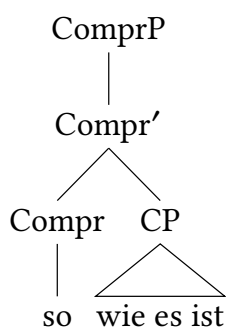
Figure 4.19: The ComprP-analysis
