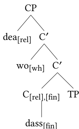
Figure 4.13: Triple combinations
