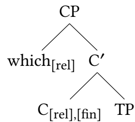
Figure 2.13: Relative operators
